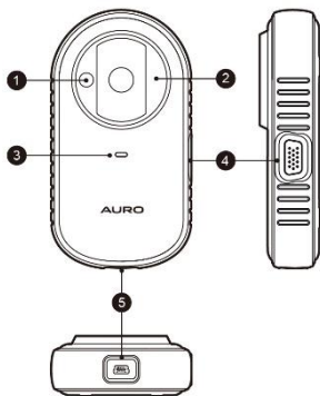
Figure 2-4 UP200 Views
